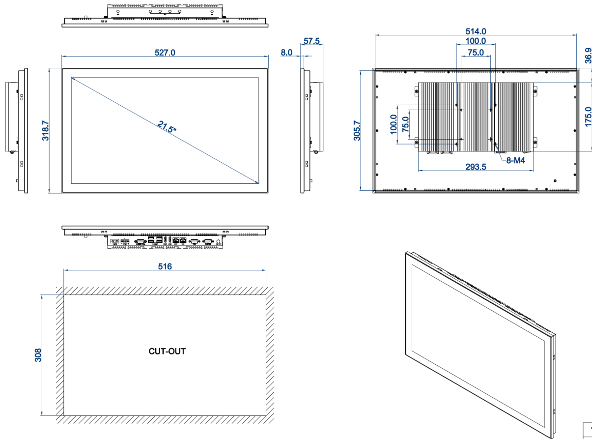
DIMENSIONAL DRAWING:TPC-DCS215
