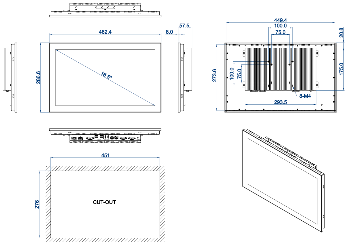
DIMENSIONAL DRAWING:TPC-DCS185
