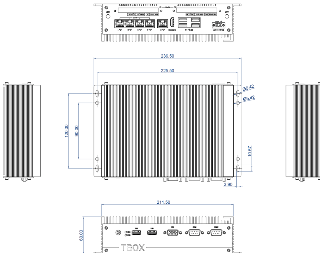
DIMENSIONAL DRAWING:TBOX-3TX0
